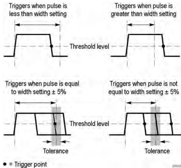
Pulse Width Trigger Conditions
