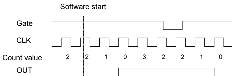
Figure 4-21: Mode 4-Single-Gated Pulse
