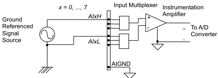
Figure 2-17: GRND-Referenced Source w/ P-D Input
