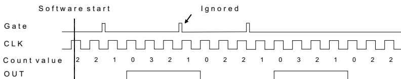
Figure 4-23: Mode 6-Re-Triggered Single Pulse
