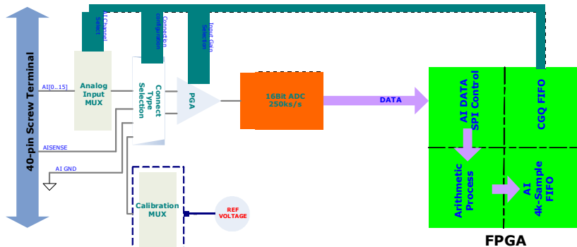
Figure 4-2: Analog Input
