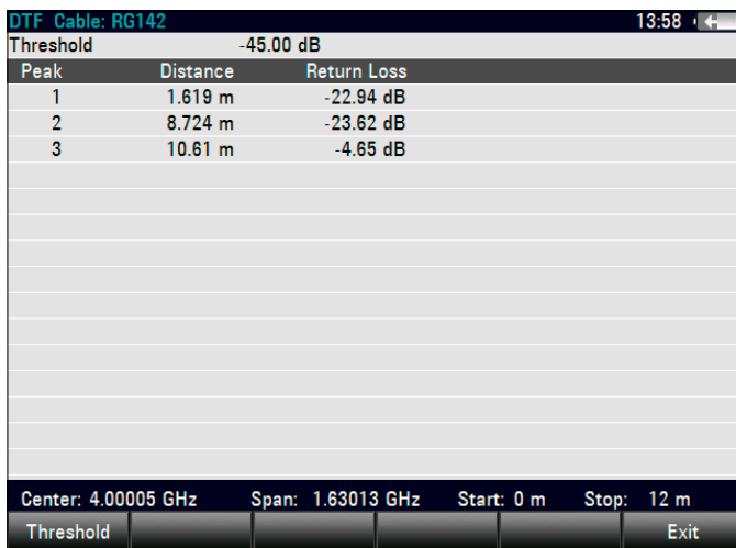
List display of cable faults that exceed a predefined threshold
