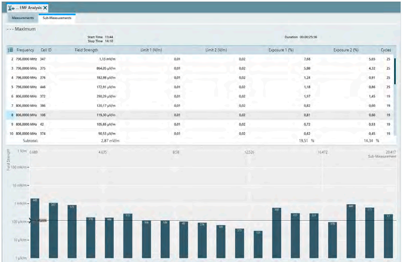
Measurement results of the R&S®FSH-K105 EMF measurement application
