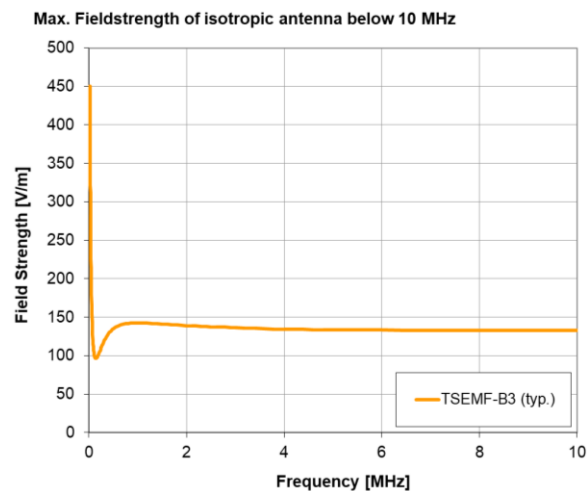
Maximum field strength for R&S®TS-EMF isotropic antennas
