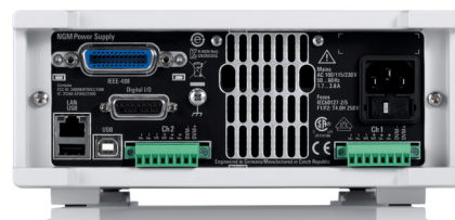
R&S®NGM202, rear view
