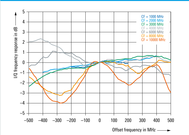
Frequency response of the I/Q modulator in the R&S®SGS100A (measured)
