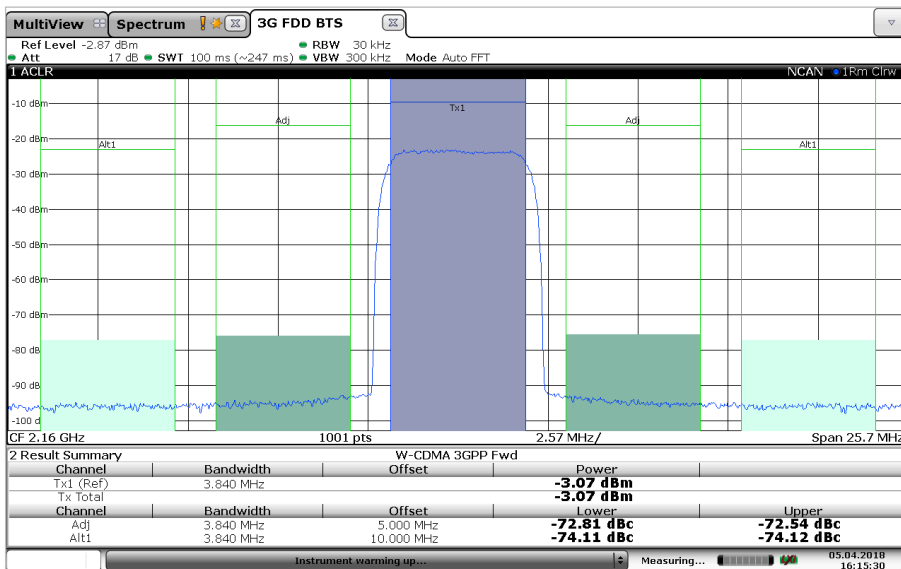
Measured ACPR for 3GPP test model 1, 64 DPCH
