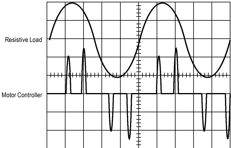
Figure 2: Typical Current Waveforms
