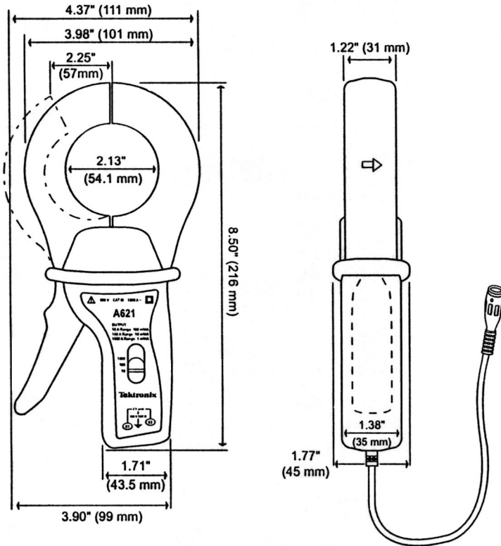
Figure 4: Physical dimensions
