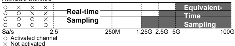
Sampling rate by number of active channels
