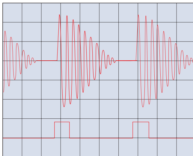
Abb. 4.2: getriggertes Arbitrary-Signal
