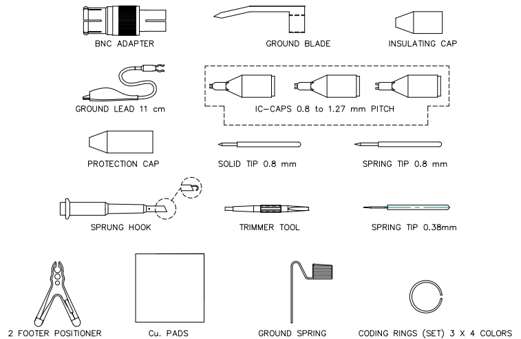
Model 6551 Microline Passive Oscilloscope Probe with Readout Actuator
